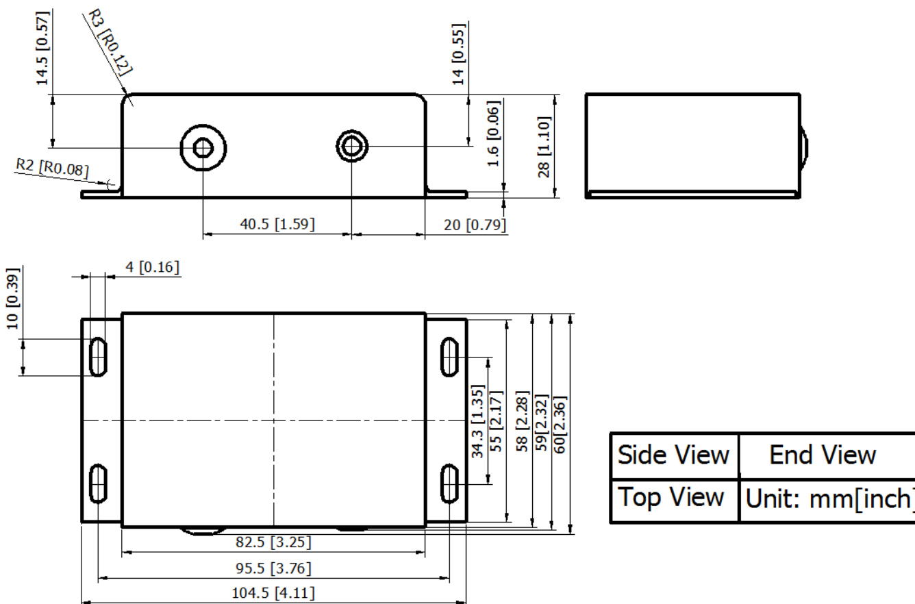
Figure 14. Outline Dimensions
