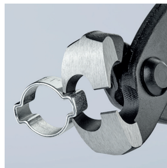
Using the side press jaw
