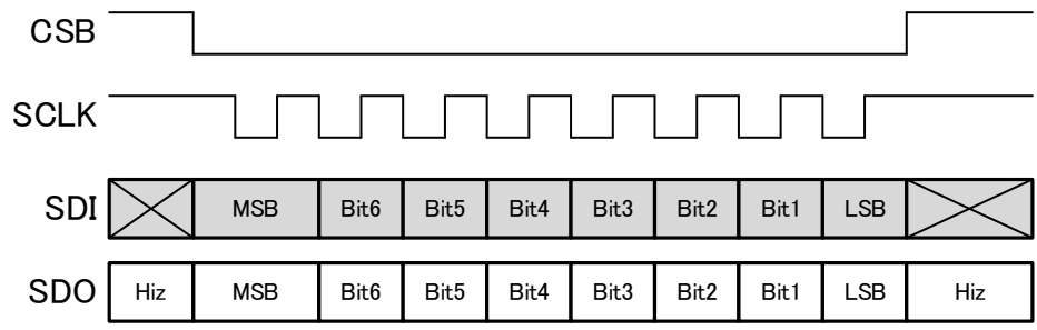
Fig. 17 SPI Waveform
