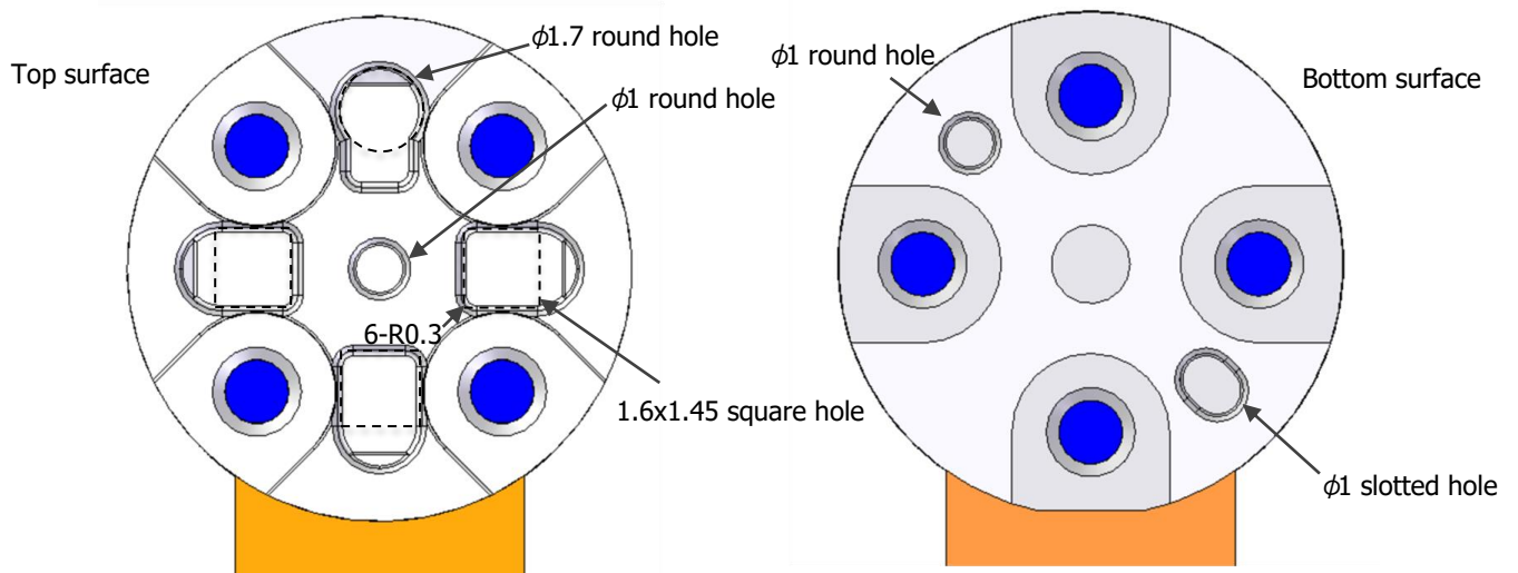
Fig. 30 Positioning holes
