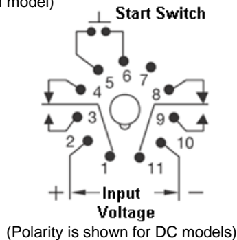
11-PIN CONFIGURATION
