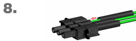
Slide shrinking tube (1) on connector shell (3)
