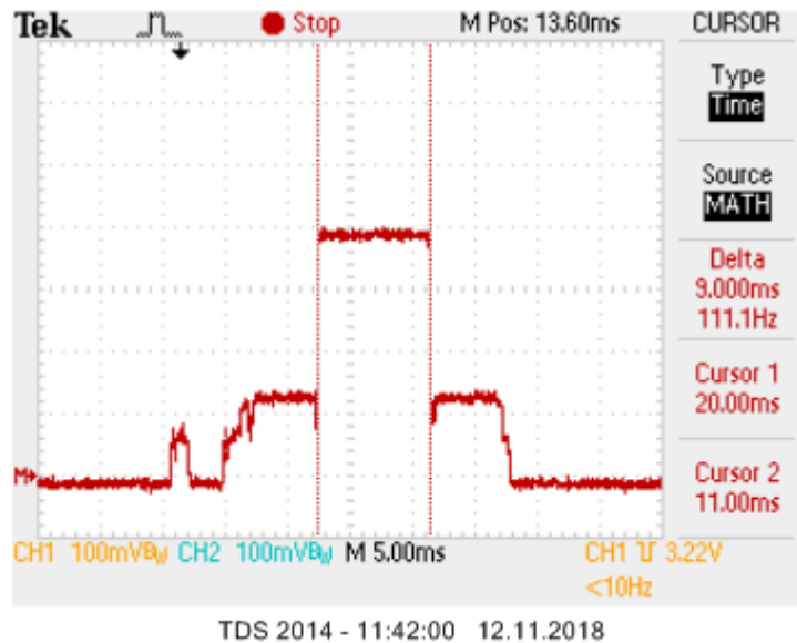
Figure 7. Current consumption transmission of 30 application bytes
