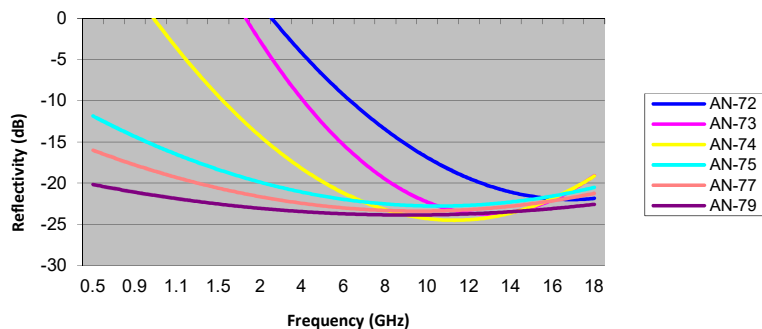
Typical Reflectivity
