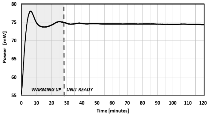
FIG. 9: WARM-UP TIME
