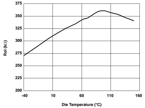
Transimpedance (Rol) vs Temperature
