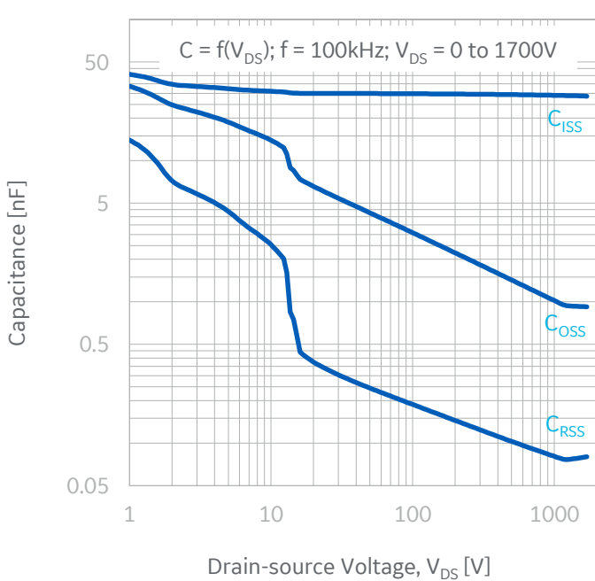
Figure 8: Junction Capacitances to 1700 V
