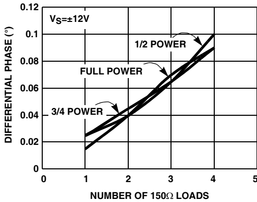
FIGURE 39. DIFFERENTIAL PHASE
