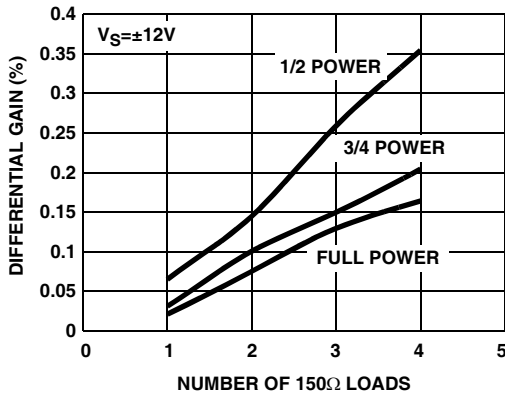
FIGURE 37. DIFFERENTIAL GAIN
